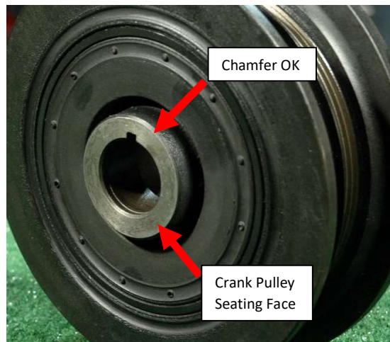
Figure 10 - R32 GTR OEM Crank Pulley 'B' (Chamfer OK)
